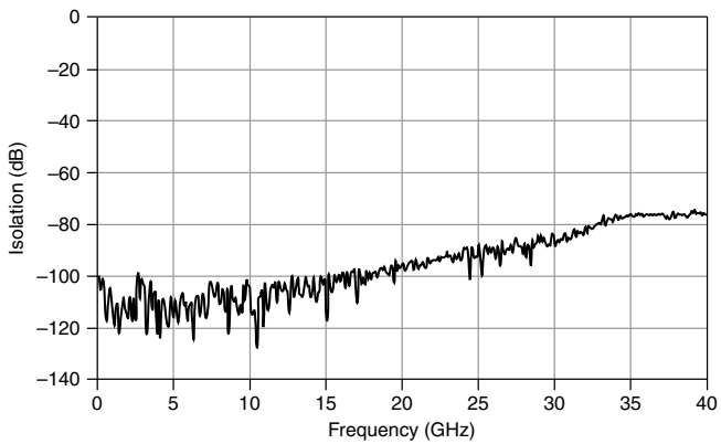
Figure 2. Typical Isolation
