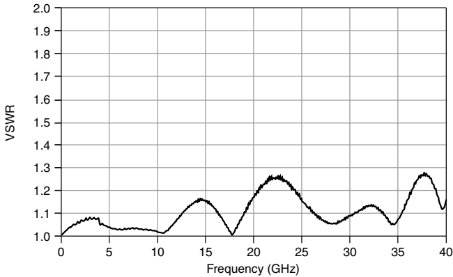
Figure 3. Typical VSWR
